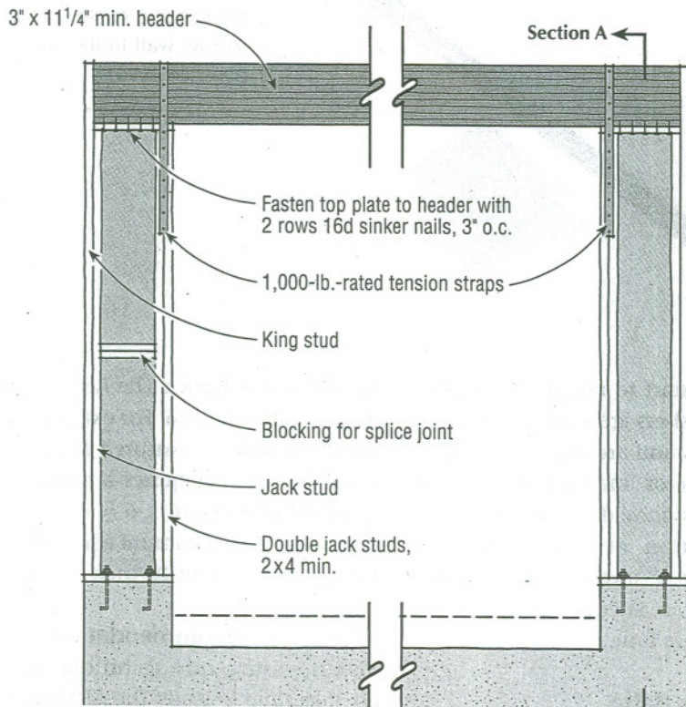
Outside Elevation
