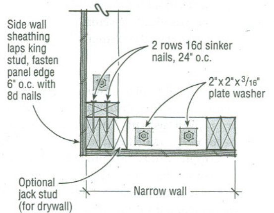
Corner Detail - Plan View
