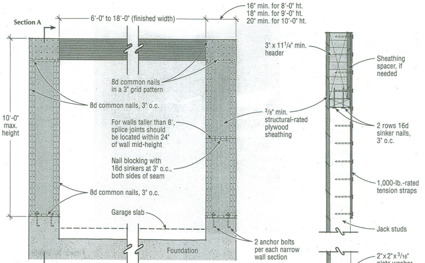
Outside Elevation
